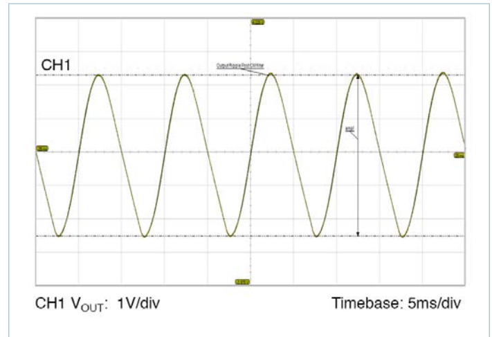
Figure 6 — Typical line frequency output voltage ripple waveform, T_{CASE} = 30^{\circ}C , V_{IN} = 230V , I_{OUT} = 6.9A , C_{OUT} = 6,800\mu F . Measured at C3, Figure 25
