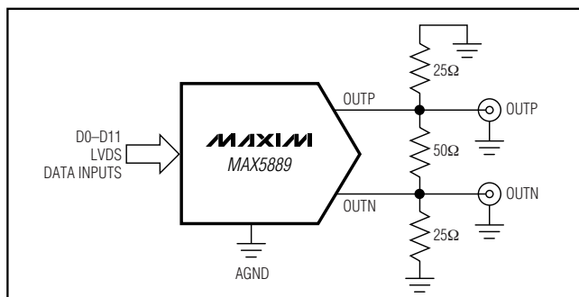
Figure 6. Differential Output Configuration
