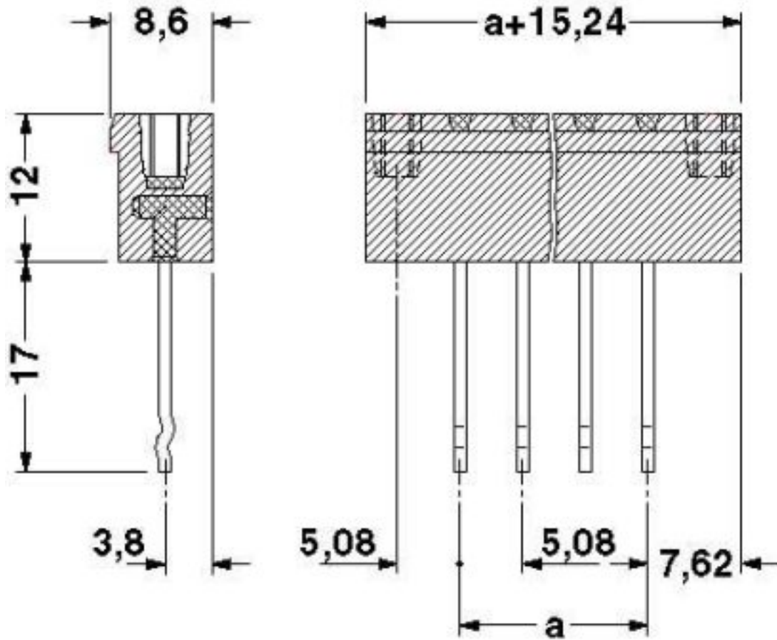
Dimensional drawing
