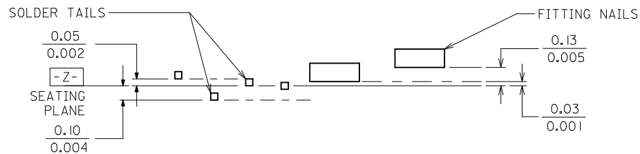
VIEW Y-Y COPLANARITY CONTROL (FOR ILLUSTRATION ONLY)
