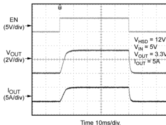
Power-Up/Power-Down
