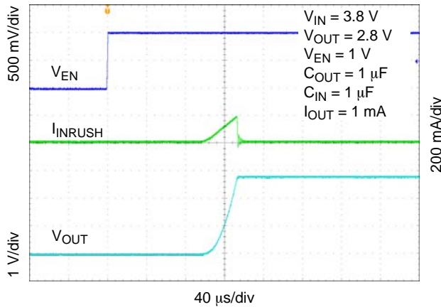
Figure 26. Enable Turn-on Response, C_{OUT} = 1 \mu\text{F} , I_{OUT} = 1 \text{ mA}
