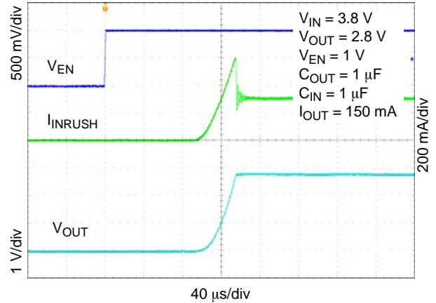
Figure 27. Enable Turn-on Response, C_{OUT} = 1 \mu\text{F} , I_{OUT} = 150 \text{ mA}
