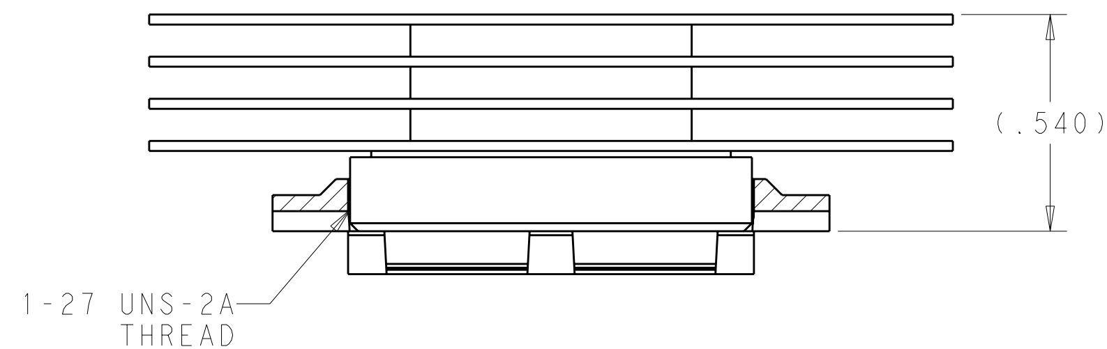
SECTION B-B
