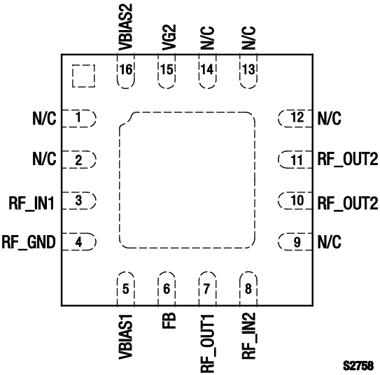
Figure 2. SKY67107-306LF Pinout – 16-Pin QFN (Top View)
