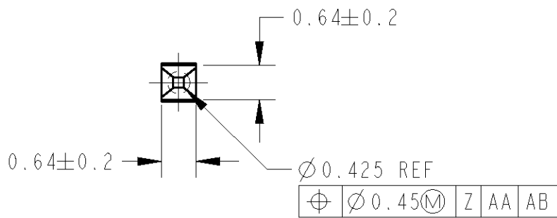
DETAIL B SCALE 10:1
