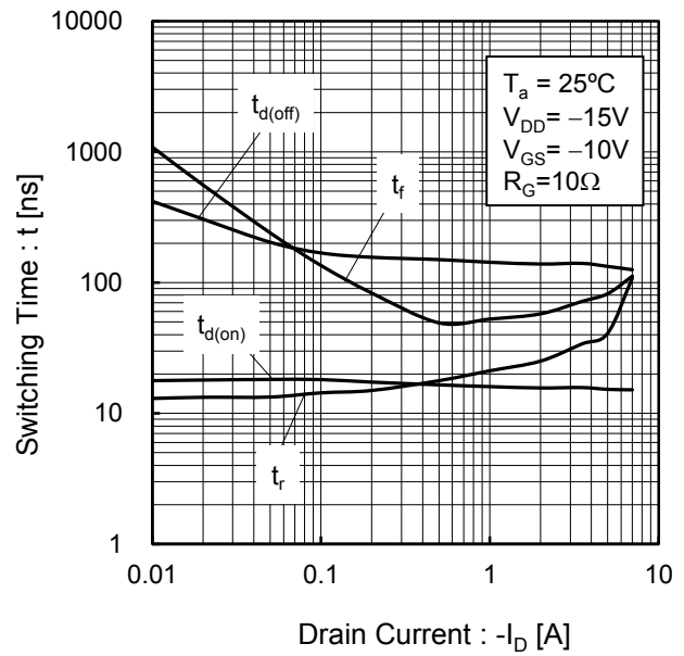
Fig.19 Switching Characteristics
