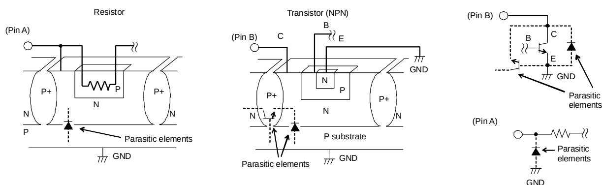
Fig.29 Example of a Simple Monolithic IC Architecture
