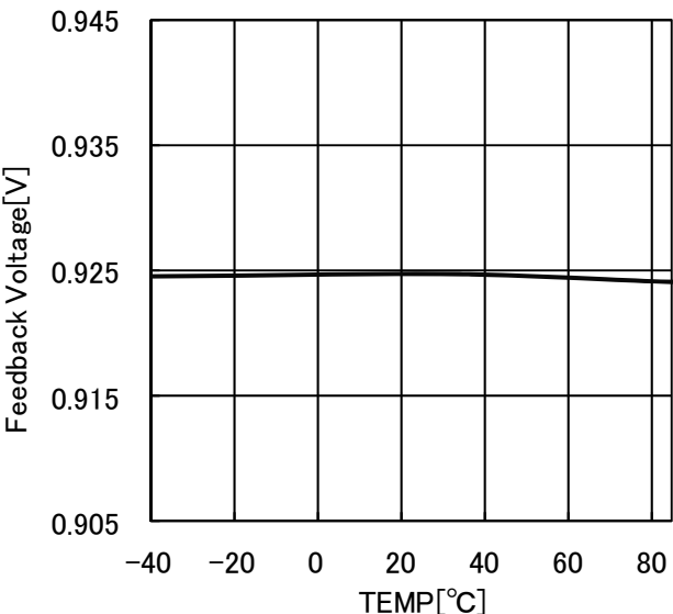
Fig.7 Feedback voltage
