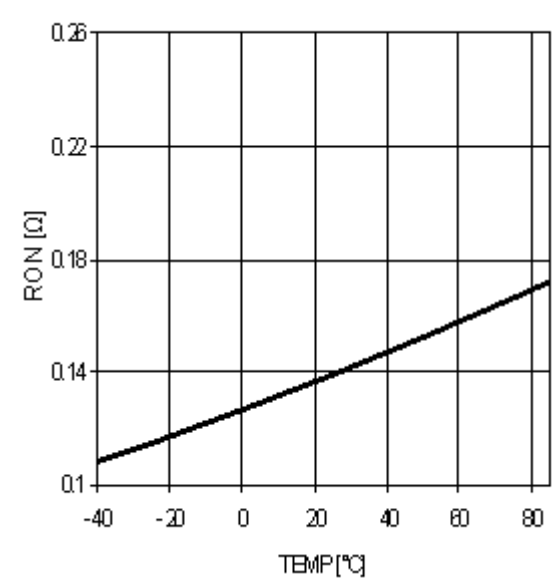
Fig.8 Hi,Low-Side On-resistance
