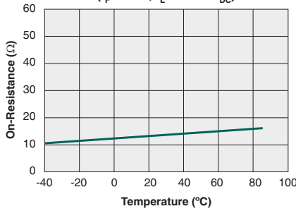
Typical On-Resistance vs. Temperature ( I_F=5mA, I_L=170mA_{DC} )
