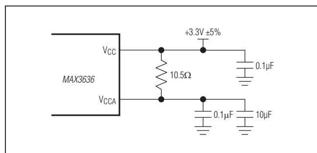
Figure 3. Power-Supply Filter
