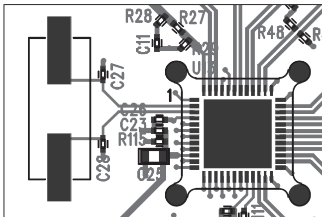
Figure 6. Crystal Layout
