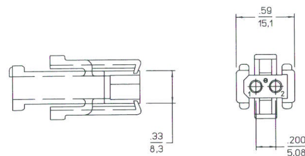
PLUG CONNECTOR SMS/SMV2P-1---
