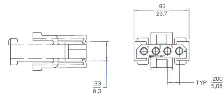
PLUG CONNECTOR SMS/SMV4P-1---
