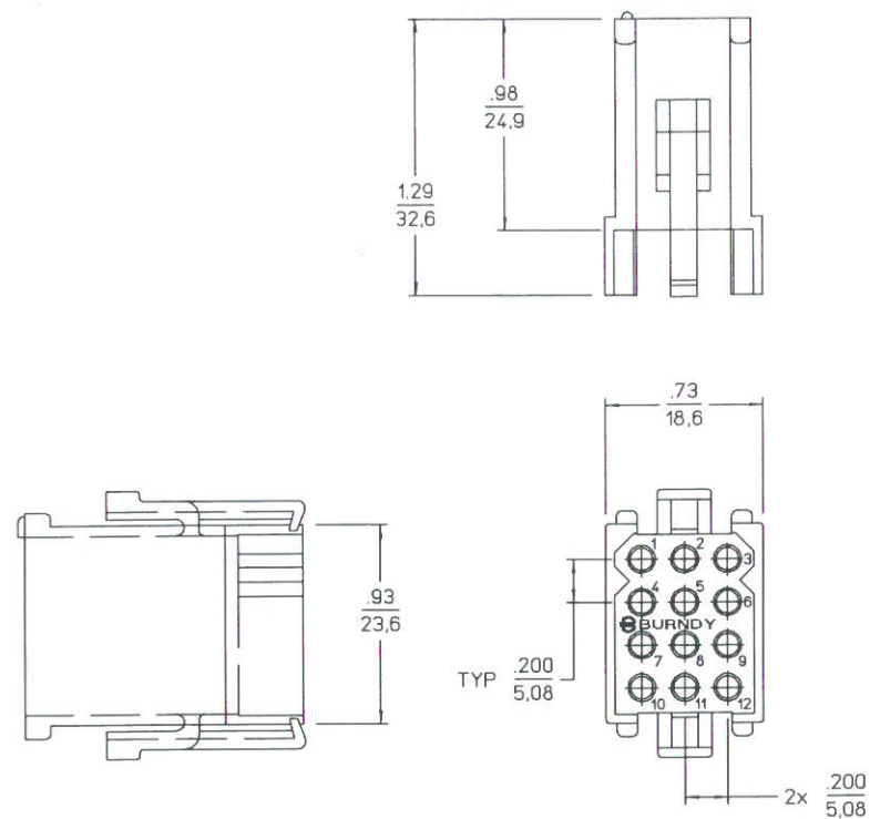
PLUG CONNECTOR SMS/SMV12P-1---
