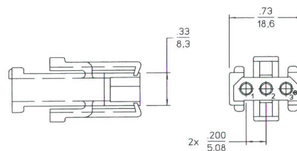
PLUG CONNECTOR SMS/SMV3P-1---
