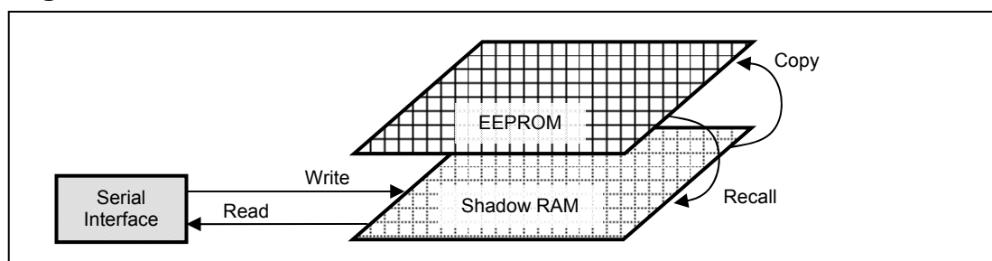
Figure 21. EEPROM Access via Shadow RAM
