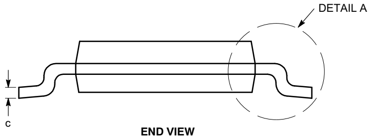
END VIEW
