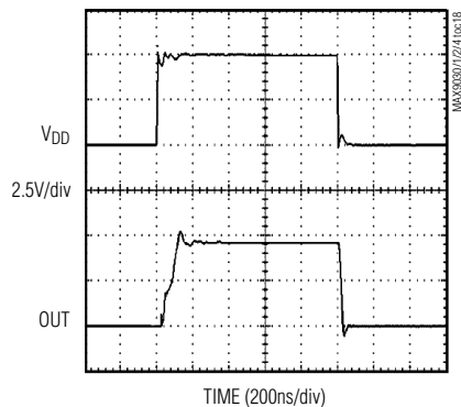
POWER-UP DELAY
