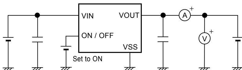
Figure 15 Test Circuit 6
