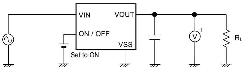
Figure 14 Test Circuit 5
