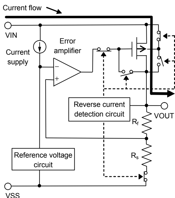
Figure 22 Normal Operation Mode
