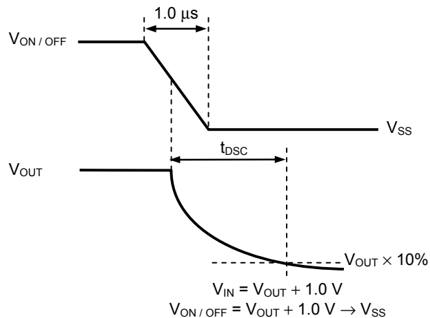
Figure 27 Test Condition of Discharge Time
