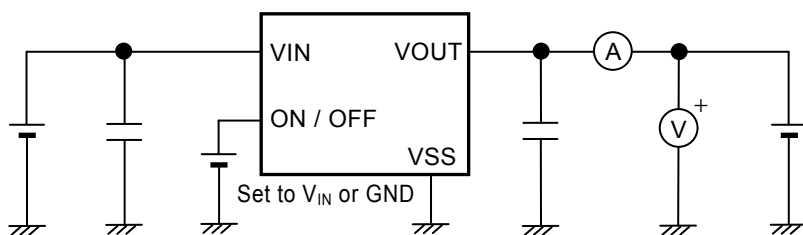
Figure 12 Test Circuit 3
