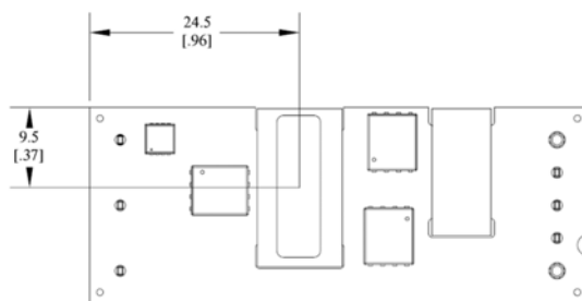
Figure 21. Pick and Place Location.
