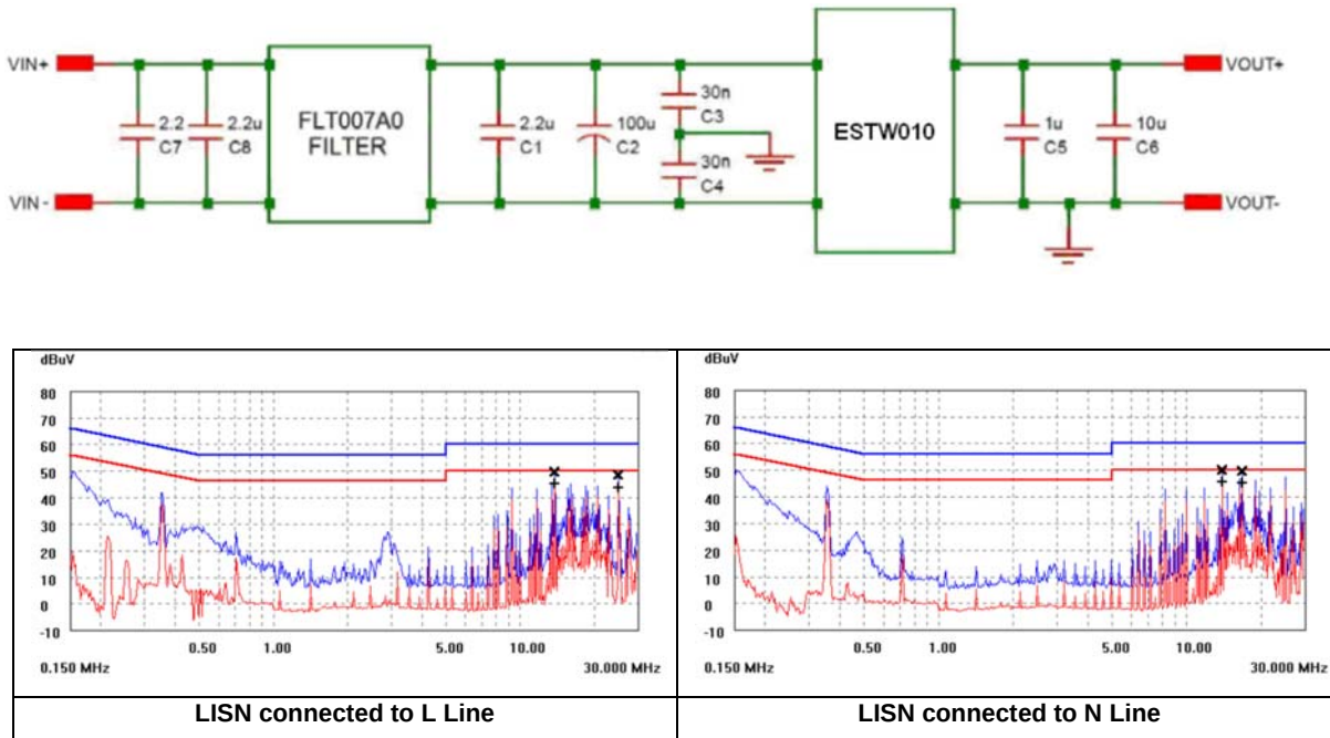
Figure 26. EMC Considerations
