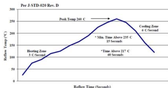
Figure 25. Recommended linear reflow profile using \text{Sn}/\text{Ag}/\text{Cu} solder.
