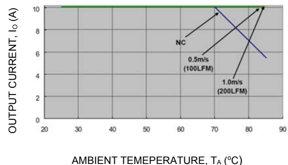
Figure 17. Output Current Derating for the Open Frame Module with Heatplate and 0.25\"/>
