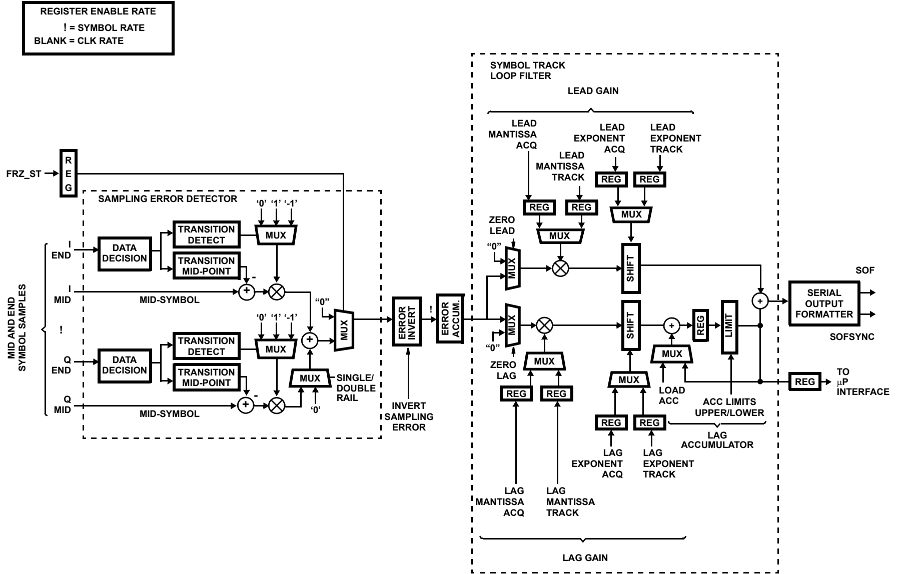
FIGURE 11. SYMBOL TRACKING
