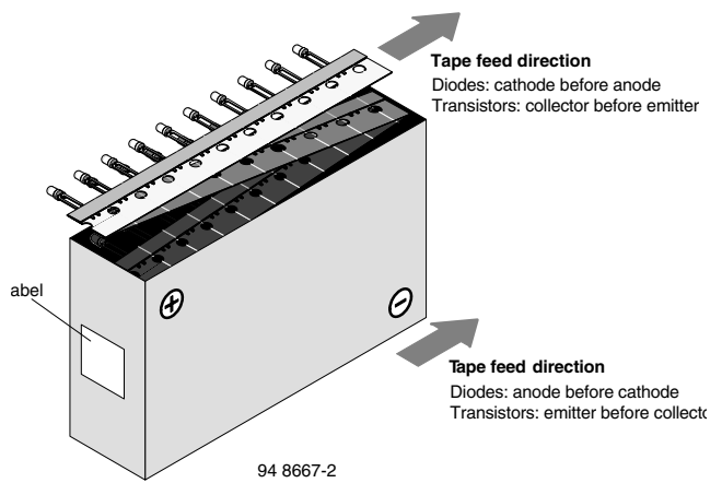
Fig. 20 - Tape Direction
