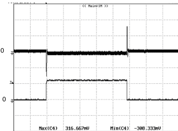
Figure 17: Typical transient response to step load change at 10A/\mu S from 50%~100% load, at 12Vin, 2.5V out
