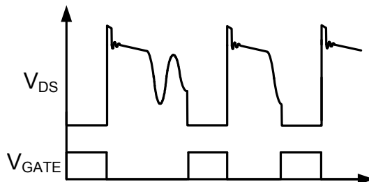
Figure 16. Valley-Skipping Mode
