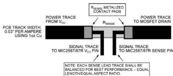
Figure 6. 4-Wire Kelvin Sense Connections for R_{\text{SENSE}}
