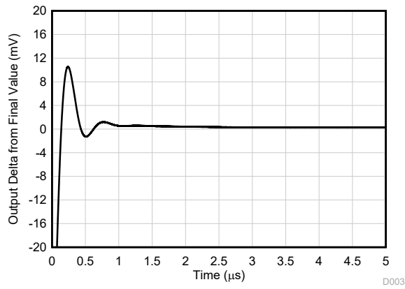
Figure 6-31. Large-Signal Step Response (Rising)
