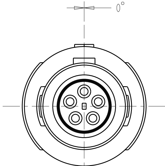
0° KEYING SCALE 4:1
