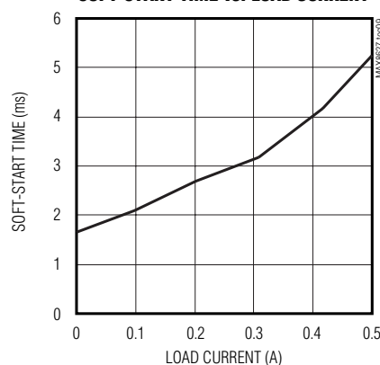
SOFT-START TIME vs. LOAD CURRENT
