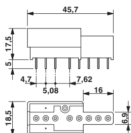
Dimensional drawing
