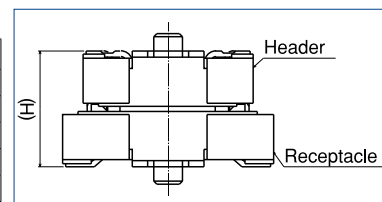
(H) : Reference dimension
