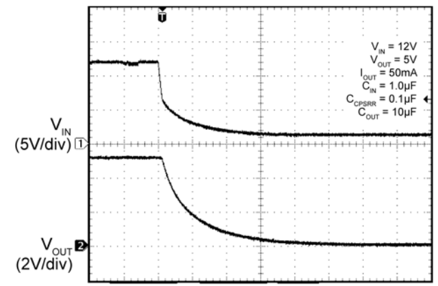
Fast Turn-Off
