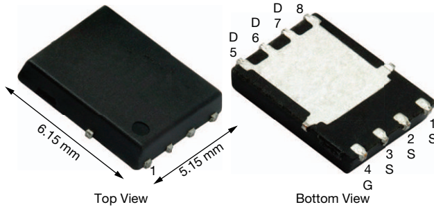
PowerPAK® SO-8 Single
