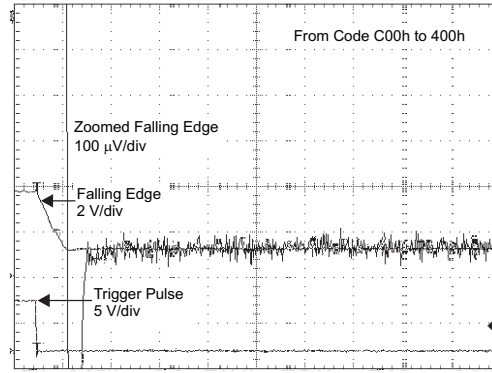
HALF-SCALE SETTLING TIME: 5V FALLING EDGE
