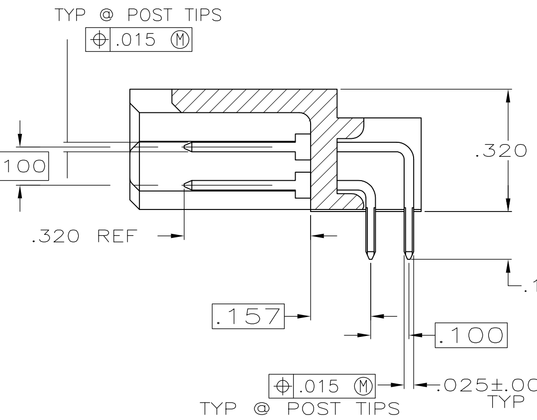
SECTION M-M
