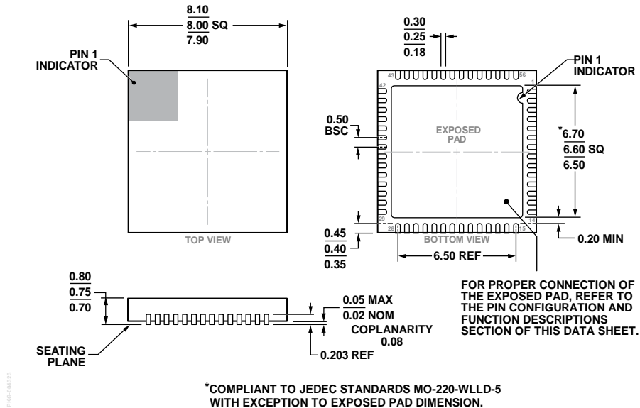
Figure 75. 56-Lead Lead Frame Chip Scale Package [LFCSP_WQ] 8 mm x 8 mm Body, Very Very Thin Quad (CP-56-9) Dimensions shown in millimeters
