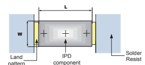
(0805 PCB footprint)
