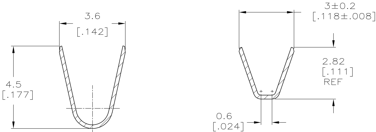
SECTION B-B
