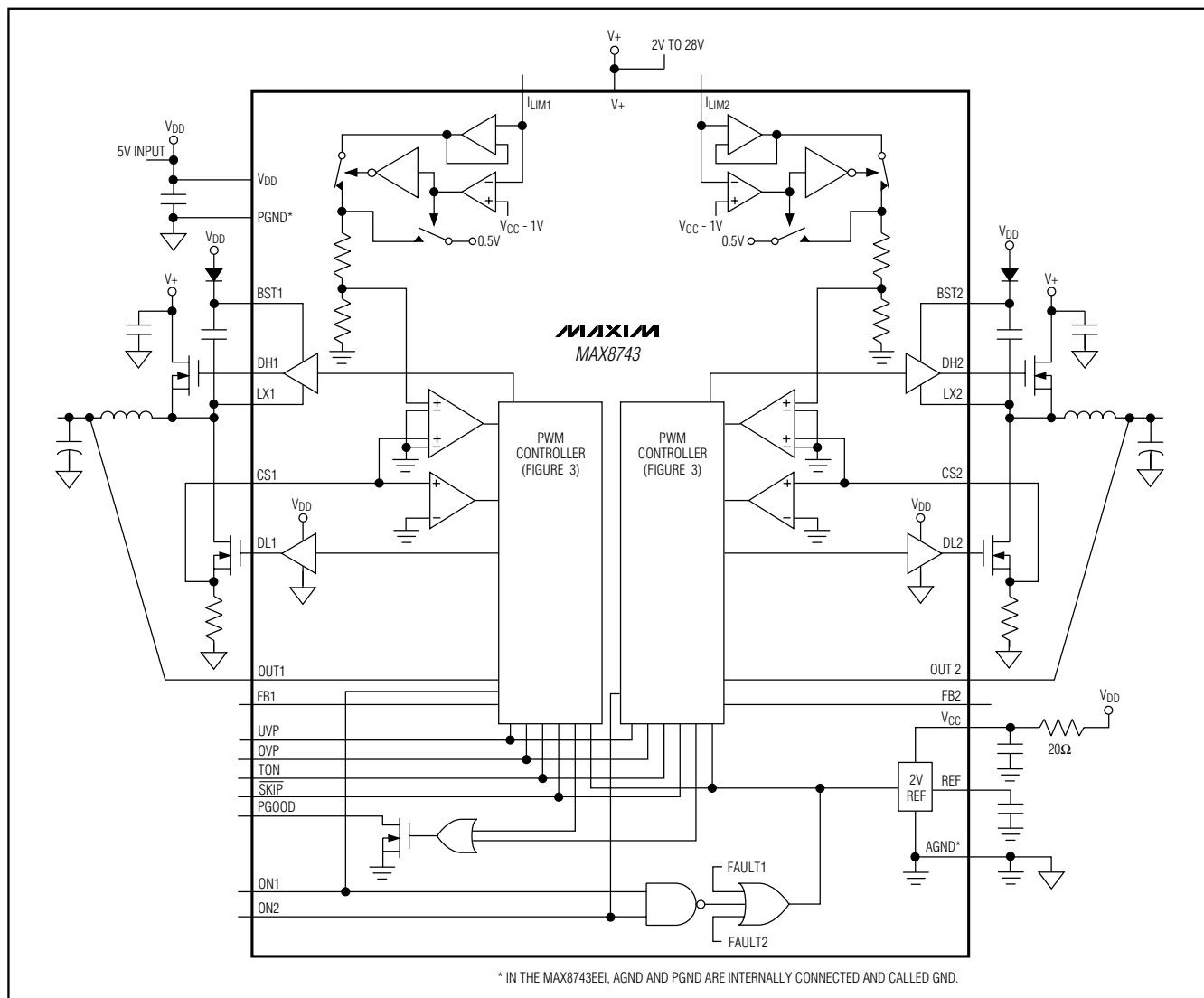
Figure 2. Functional Diagram
