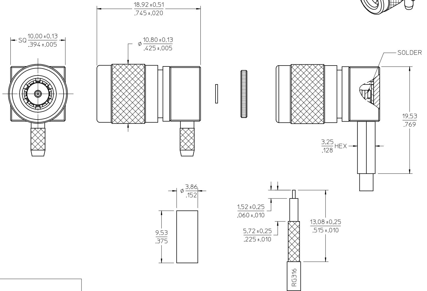
STRIPPING DIMENSIONS
