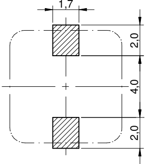
no sensitive traces underneath the component Scale - 2:1
