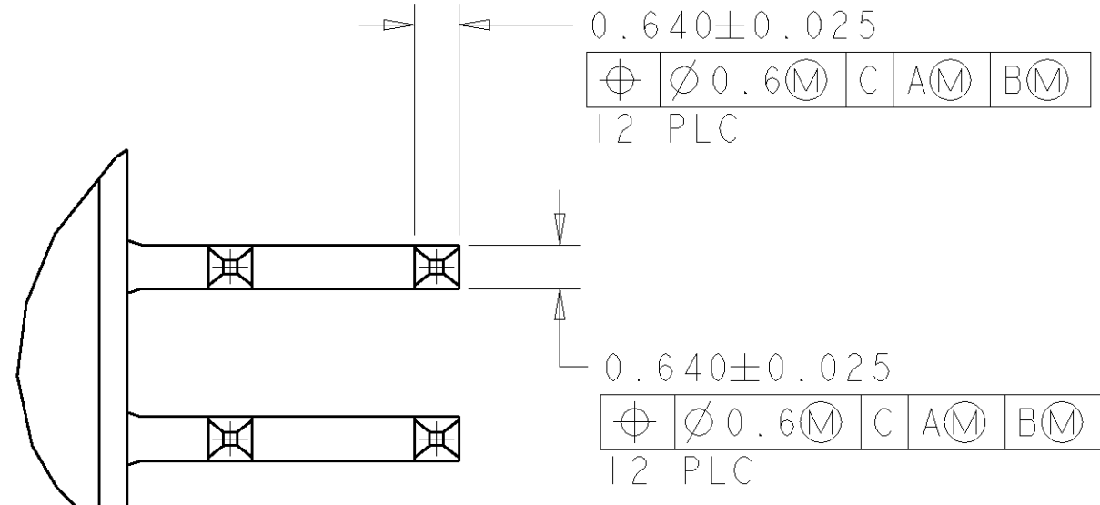
DETAIL C SCALE 10:1
