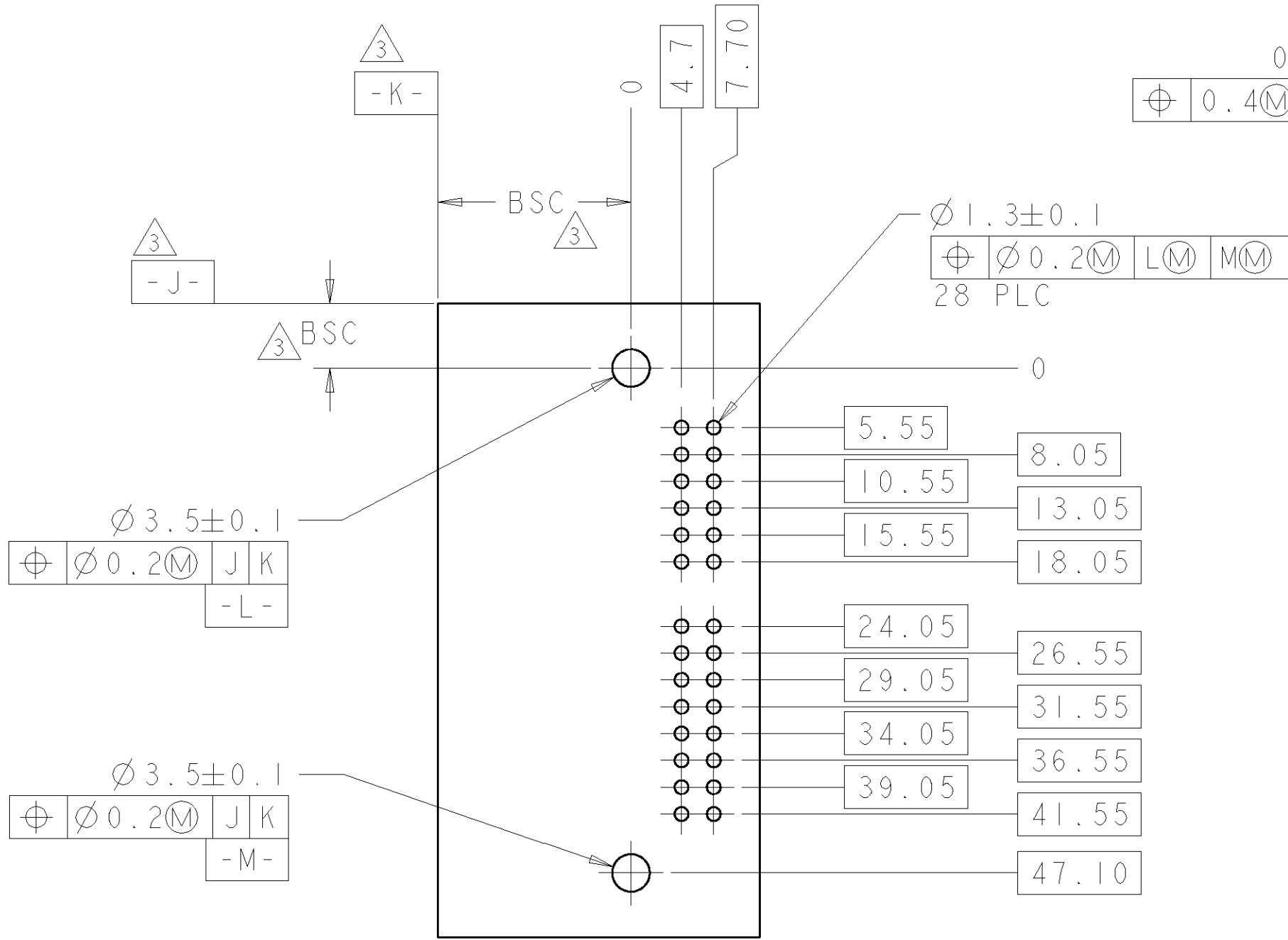
PC BOARD LAYOUT RECOMMENDED THICKNESS: 1.6MM
