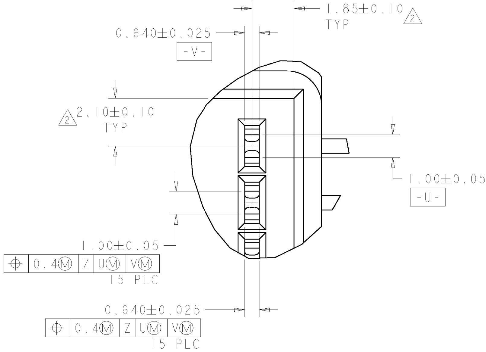
DETAIL D SCALE 10:1
