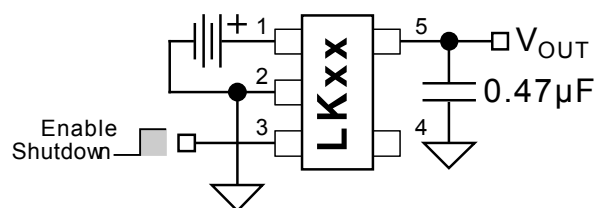
SOT-23-5 Version
