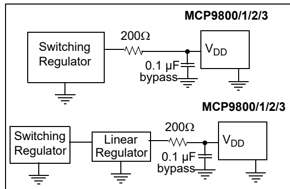
FIGURE 6-3: Power-supply Filter Using a Single Resistor.
