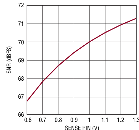
LTC2265-12: SNR vs SENSE, f_{IN} = 5\text{MHz} , -1dBFS
