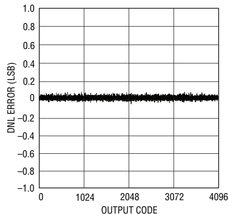
LTC2264-12: Differential Nonlinearity (DNL)
