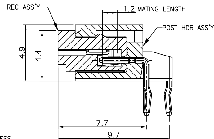
MATING SECTION
