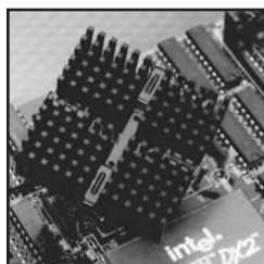
669 SERIES SpiderClip™ Heat Sink Assembly for Intel®DX4™, AMD AM486DX2, and AM486DX4 661 SERIES Heat Sink without clip
