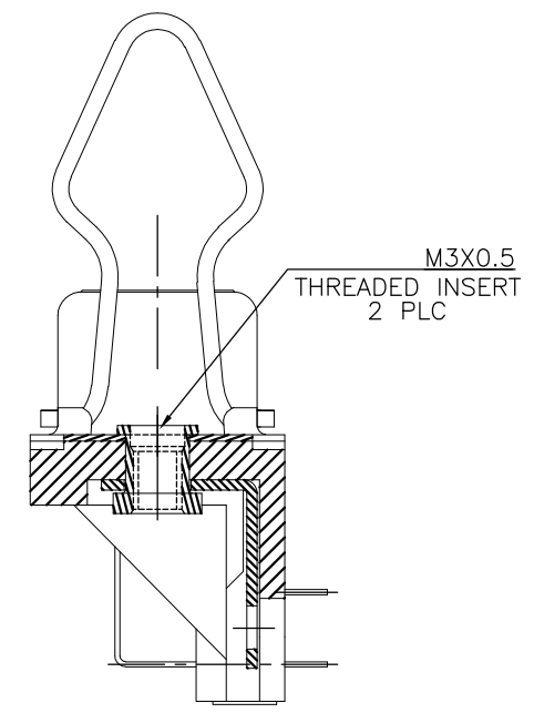
SECTION F-F
