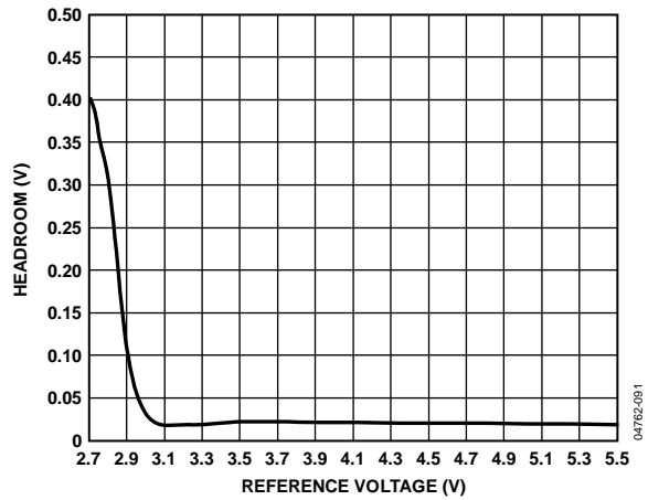
Figure 27. V_{DD} Headroom vs. Reference Voltage
