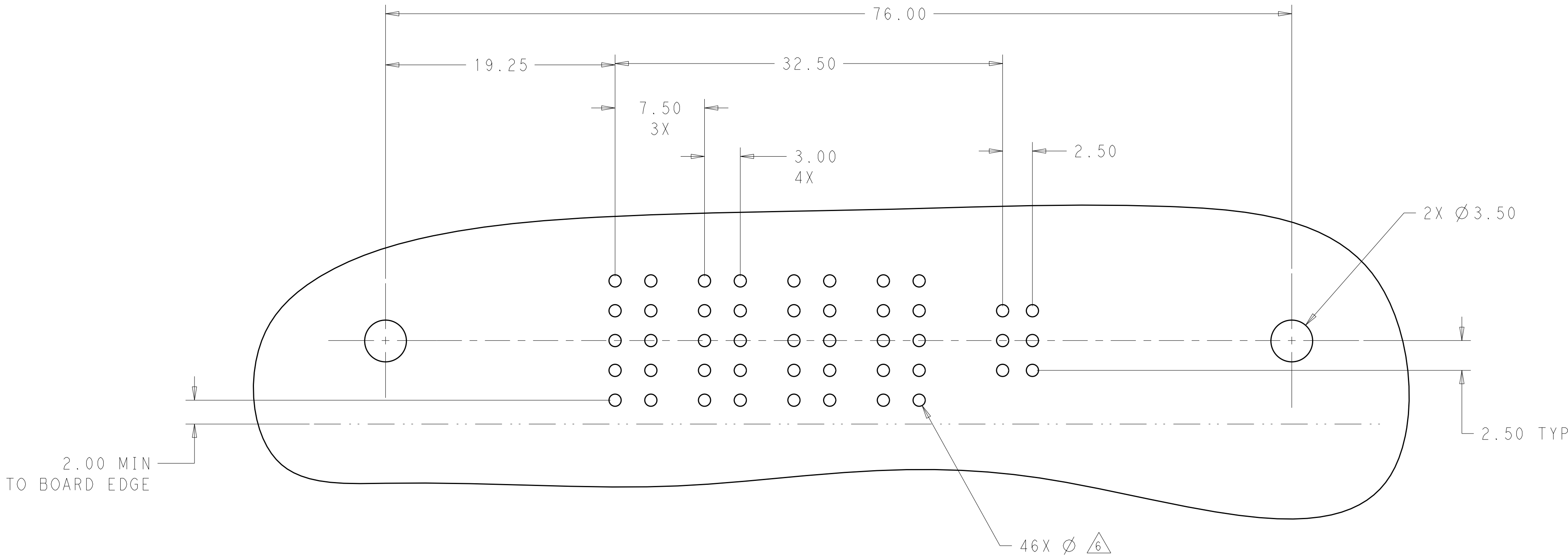
PRINTED CIRCUIT LAYOUT COMPONENT SIDE
