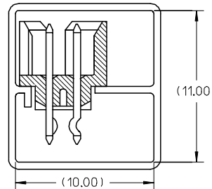
FIG. 1 : ORIENTATION OF PART IN TUBE.
