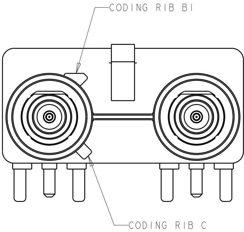
DETAIL V
