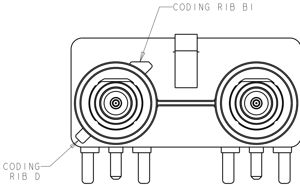
DETAIL W
