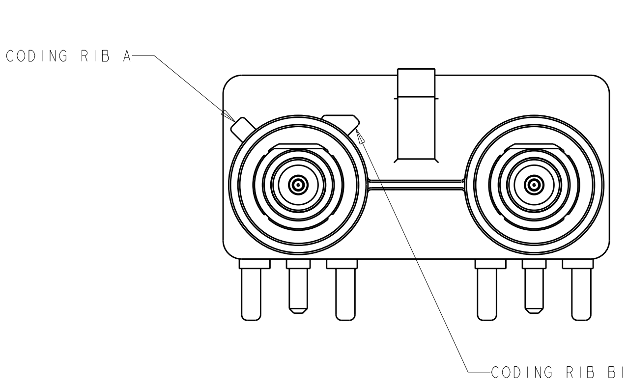
DETAIL L
