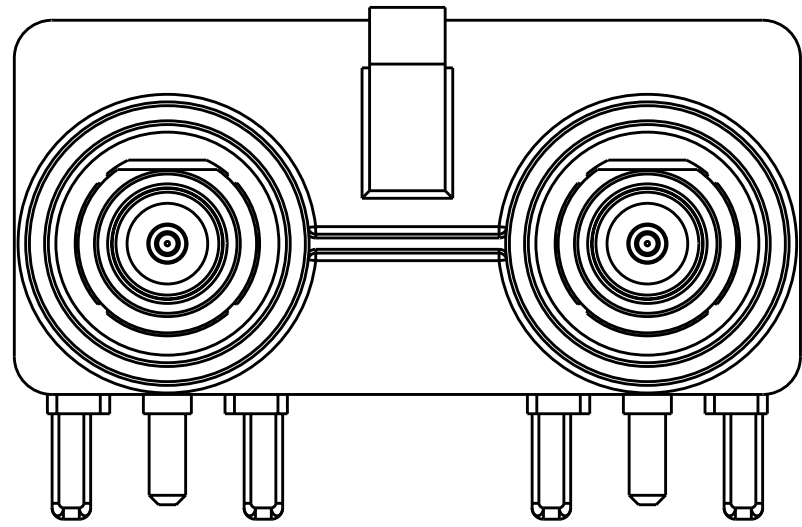
DETAIL Z
