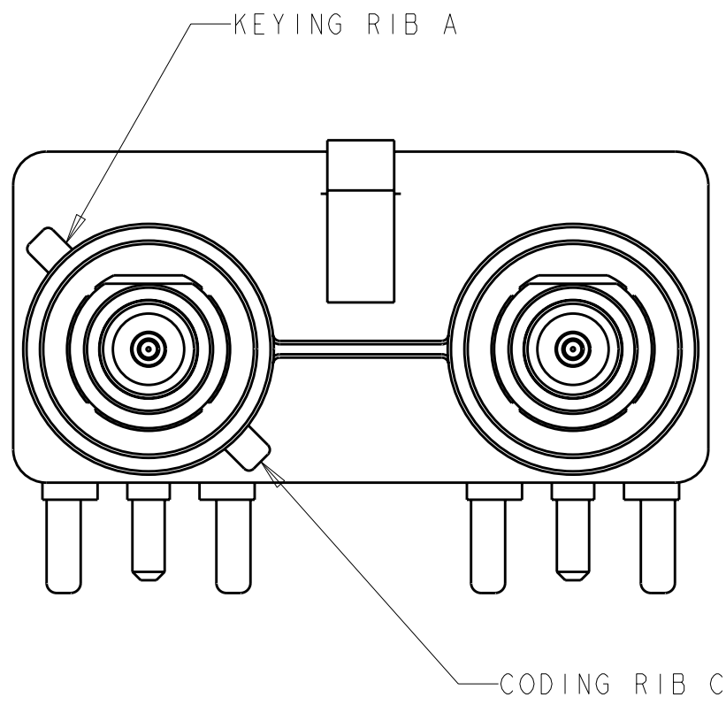
DETAIL S
